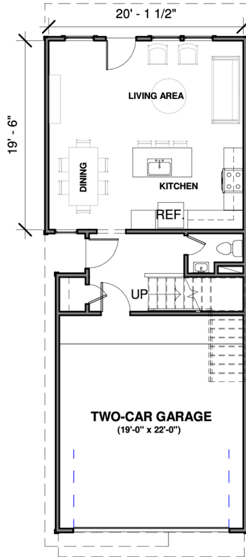
1/ First Floor 1" = 10'-0" Living Area= 601 SF
