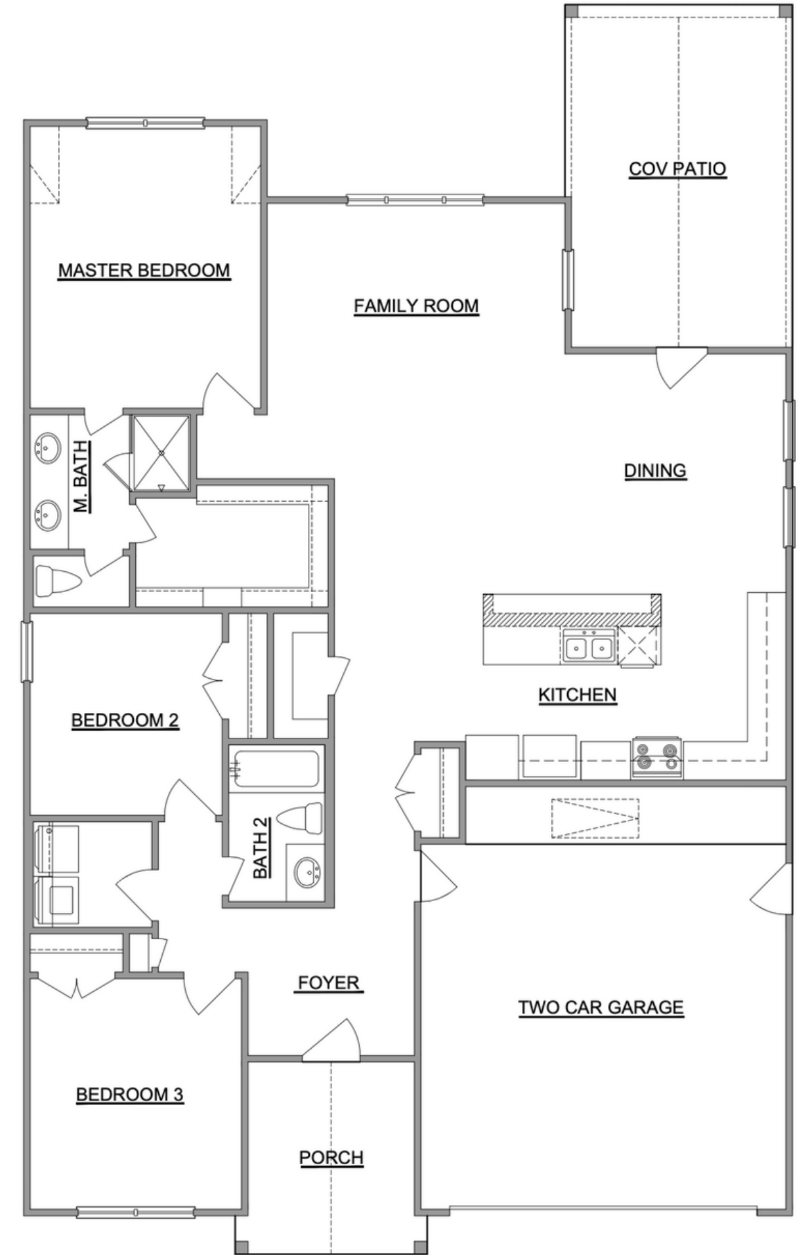
FLOOR PLAN
